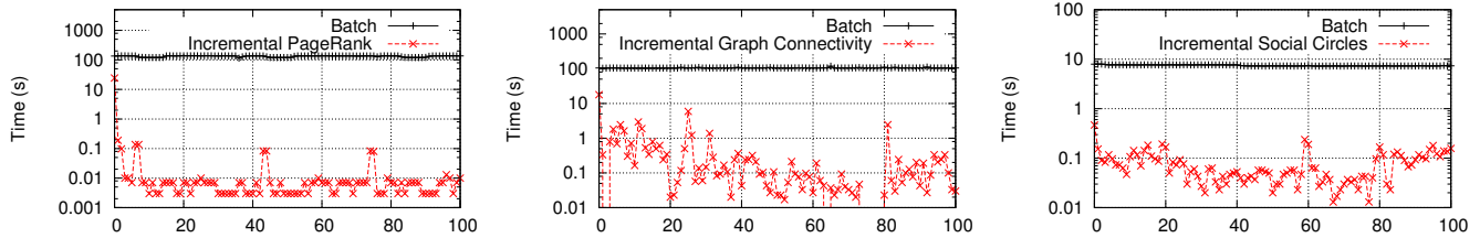
Figure 17. (left) PageRank: 100 trials ( x -axis) of deleting 1,000 edges; (center) Connectivity: 100 trials of deleting a vertex; (right) Approximate social-circle size: 100 trials of deleting 20 edges. Note: y -axis is in log-scale.
