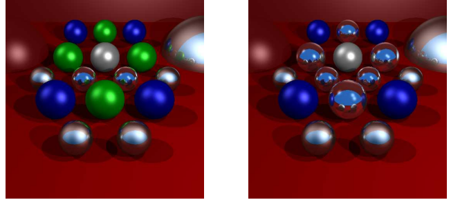
Figure 8. Two images produced by our ray tracer. To produce the right-hand image, we change the surfaces of the four green balls from diffused surfaces to mirrored surfaces. Performing change propagation yields about a 2× speedup over re-computing the output.
