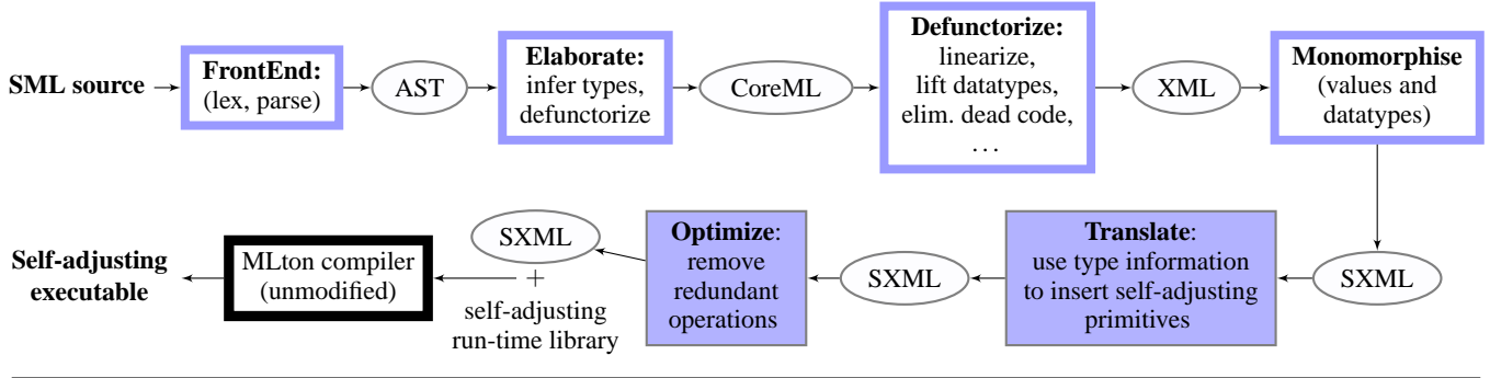
Figure 3. The structure of our compiler: new phases , modified phases , unmodified phases , intermediate languages
