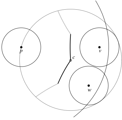
Figure 4: The points v and w are \ell -satellites of an input vertex p . Each of the hyperbolic thick curves depicts the locus of the points whose distance to an \ell -satellite is 2^{\ell-2} less than its distance to p . The Voronoi cell of p is a subset of the weighted Voronoi cell of p defined by these hyperbolic curves.
