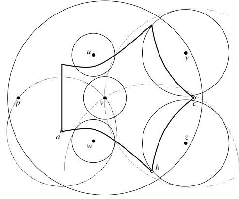
Figure 5: Illustration of the \frac{9}{2} -well-spacedness of a converted (\ell - 1) -satellite v of an input vertex p . The weighted Voronoi cell defined by the thick hyperbolic curves bound the Voronoi cell of v .
