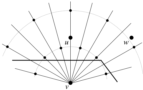
Figure 2: Zooming in on the point set M of Figure 1, first two orbits and some rays of v (nucleus) are displayed, with part of its Voronoi cell in thick lines. Intersections of odd rays with orbits at odd ranks and even rays with orbits at even ranks form satellites—potential Steiner vertices—shown in smaller dots.
