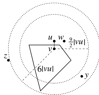
Figure 1: Given the set M = \{v, u, w, y, z\} , the nearest neighbor distance of v , \text{NN}_M(v) , is |vu| . Thick lines depict the Voronoi cell of v , \text{Vor}_M(v) ; v is 6-well-spaced, but not \frac{9}{2} -well-spaced.
